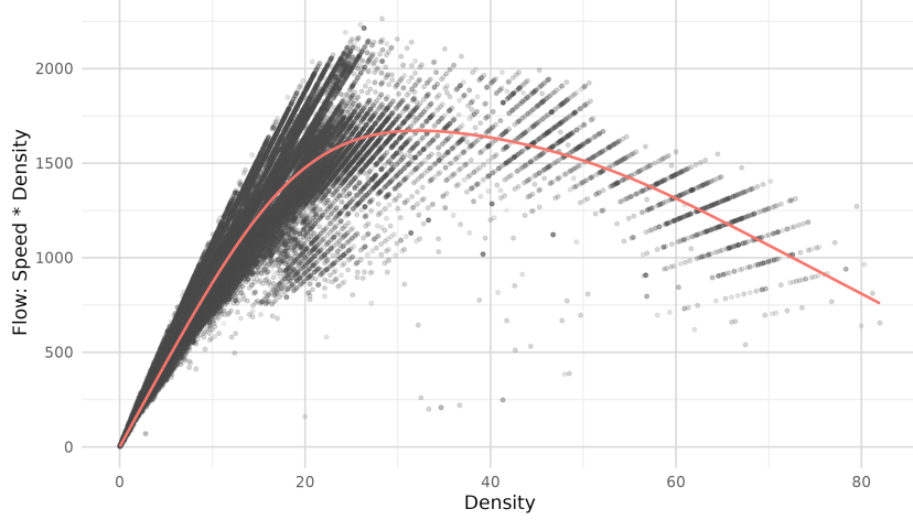
Figure 9: An estimated congestion function relating traffic flow on a segment of the Ayalon highway to traffic density on that segment.
