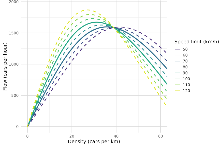
Appendix Figure F2: Extrapolated flow-density functions
